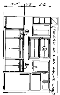
ELEVATION "A" SCALE 0 2 4 6 FT.
