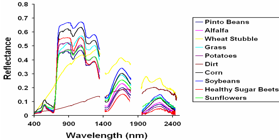
Figure 2. Spectral signatures of crops and soil. (Kyllo, 2003).
