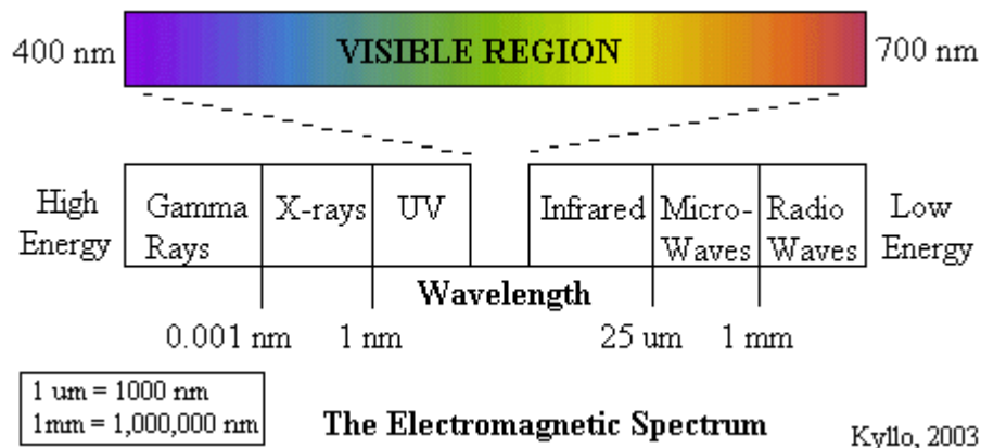
Figure 1. The visible region of the spectrum ranges from about 0.4 \mu\text{m} to 0.7 \mu\text{m} .
