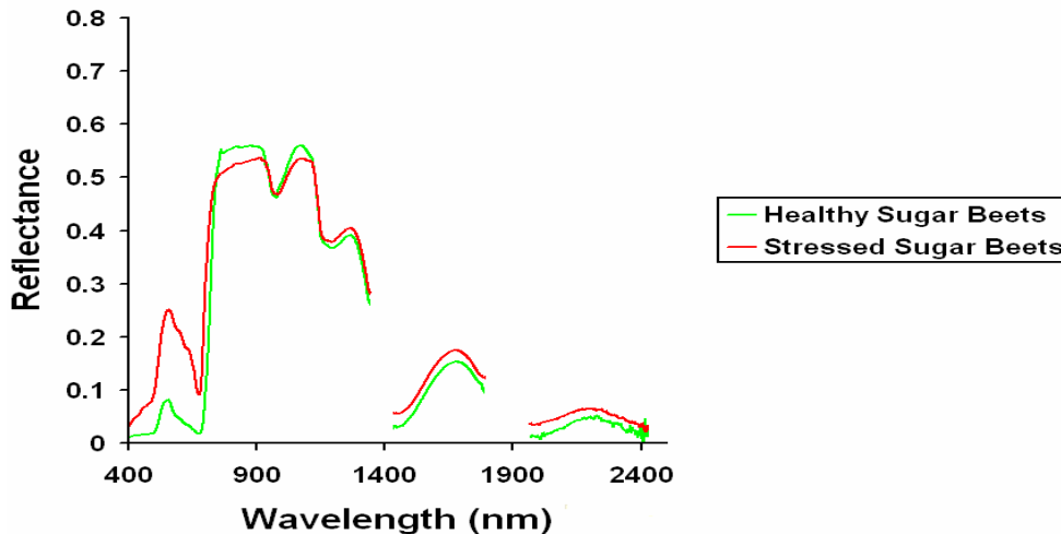
Figure 3. Spectral signatures of healthy and stressed sugarbeets. (Kyllo, 2003).
